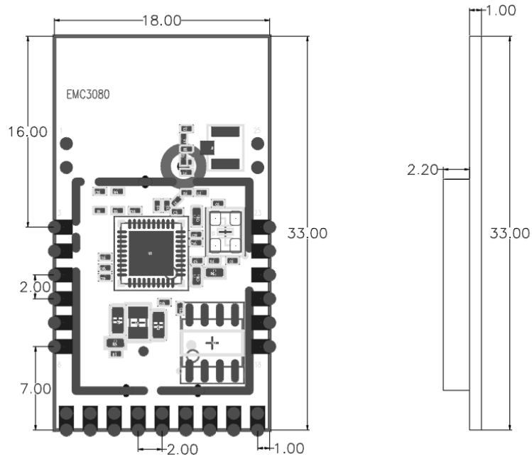
Figure 7 Assembly Dimension Diagram (unit: mm, tolerance: \pm 0.1 , outside tolerance \pm 0.2 )
